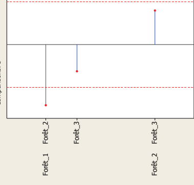
Pairwise Comparisons Comparisons: 3
