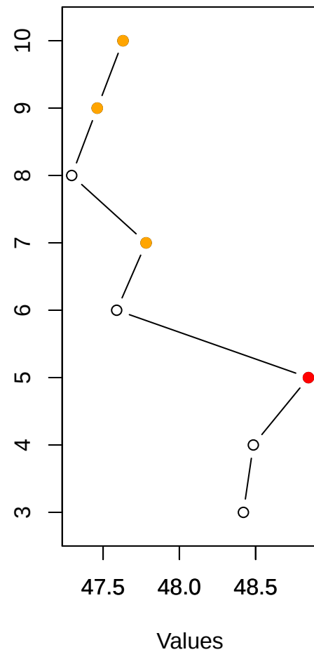
calinski criterion
