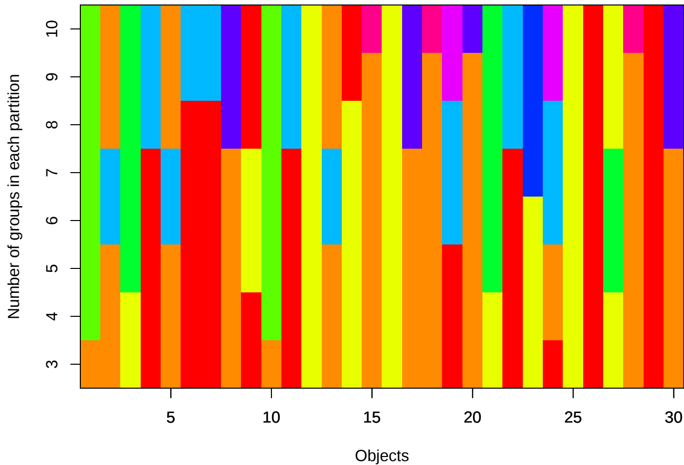
K-means partitions comparison
