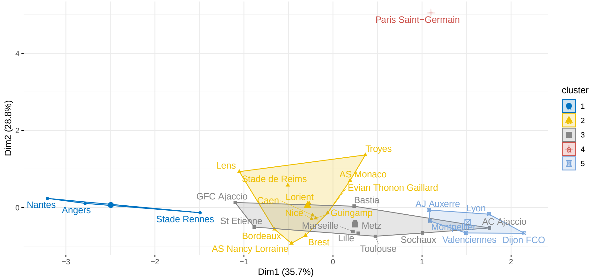
Factor map
