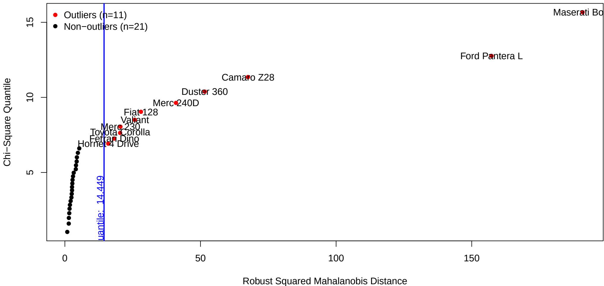
Adjusted Chi-Square Q-Q Plot
